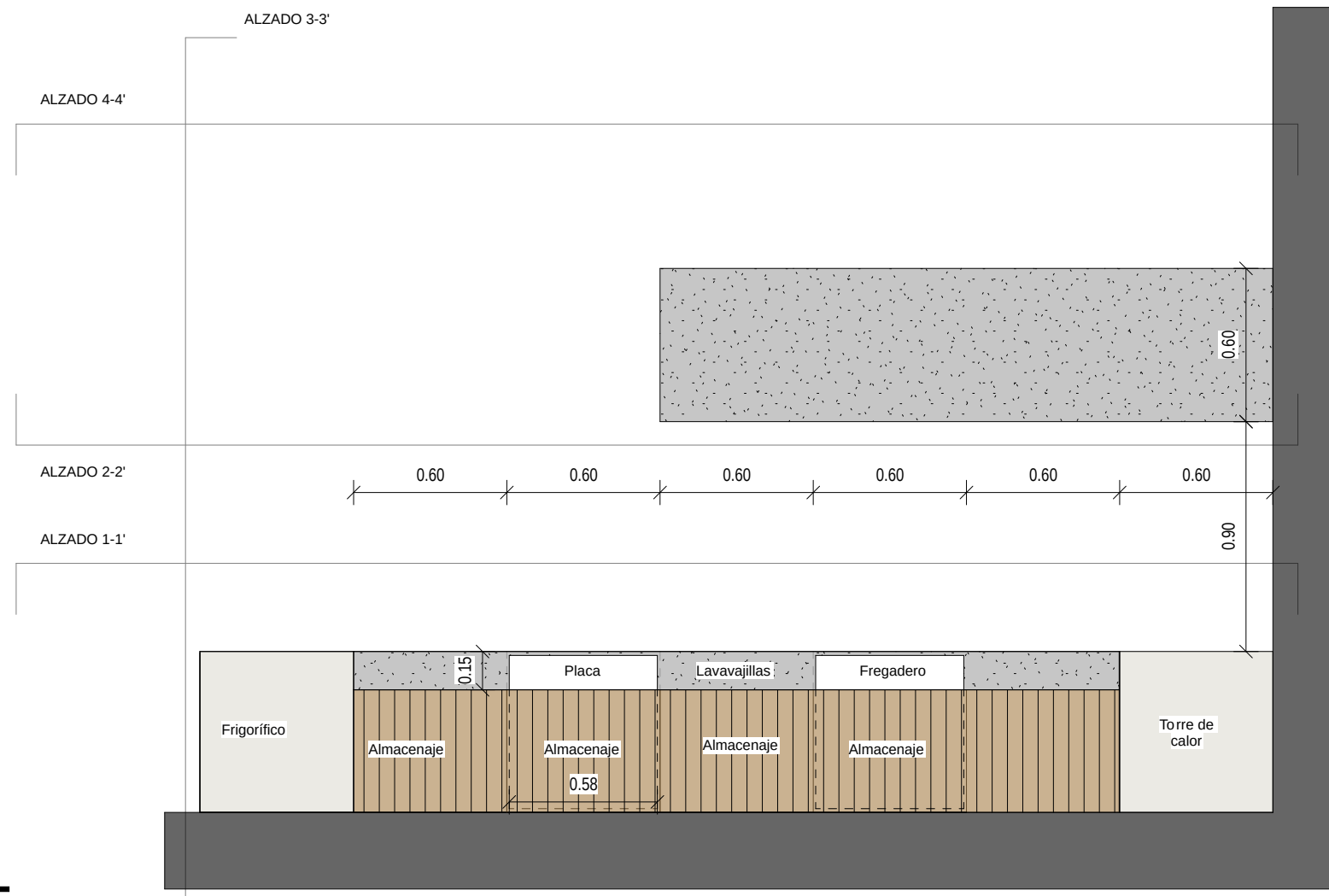
PLAN VIEW
