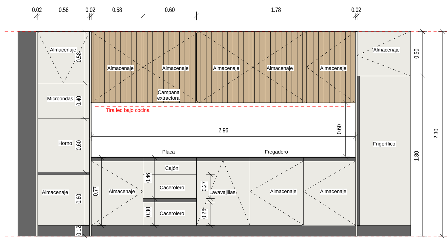
FRONT ELEVATION
